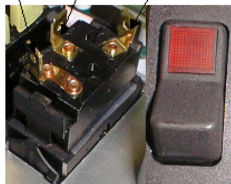
Wire Connections
