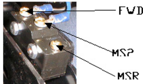
Wire Connection
