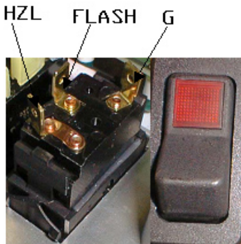
Wire Connections
