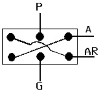
Schematic
