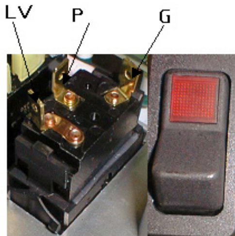
Wire Connections
