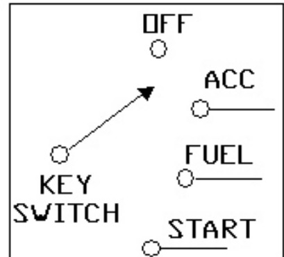
Schematic
