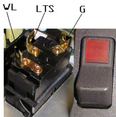
Wire Connections
