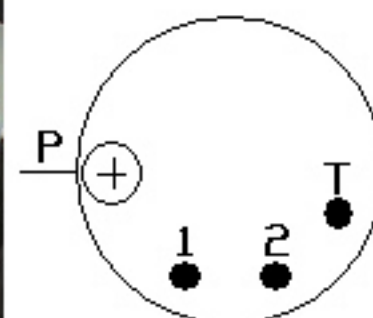
Schematic
