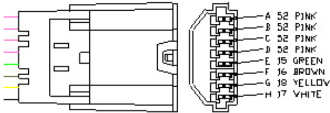
Wire Connections
