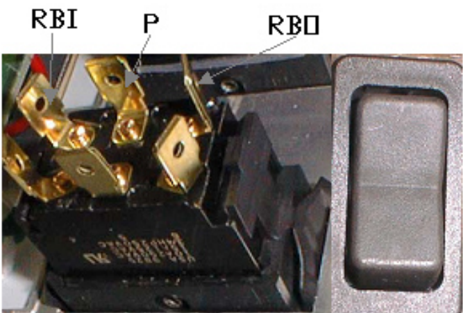
Wire Connections
