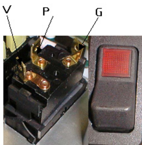
Wire Connections
