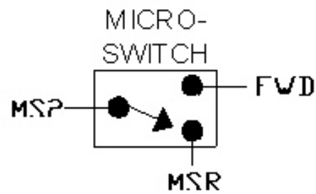
Schematic
