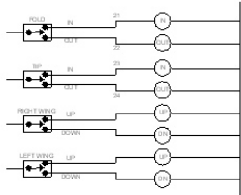
Schematic
