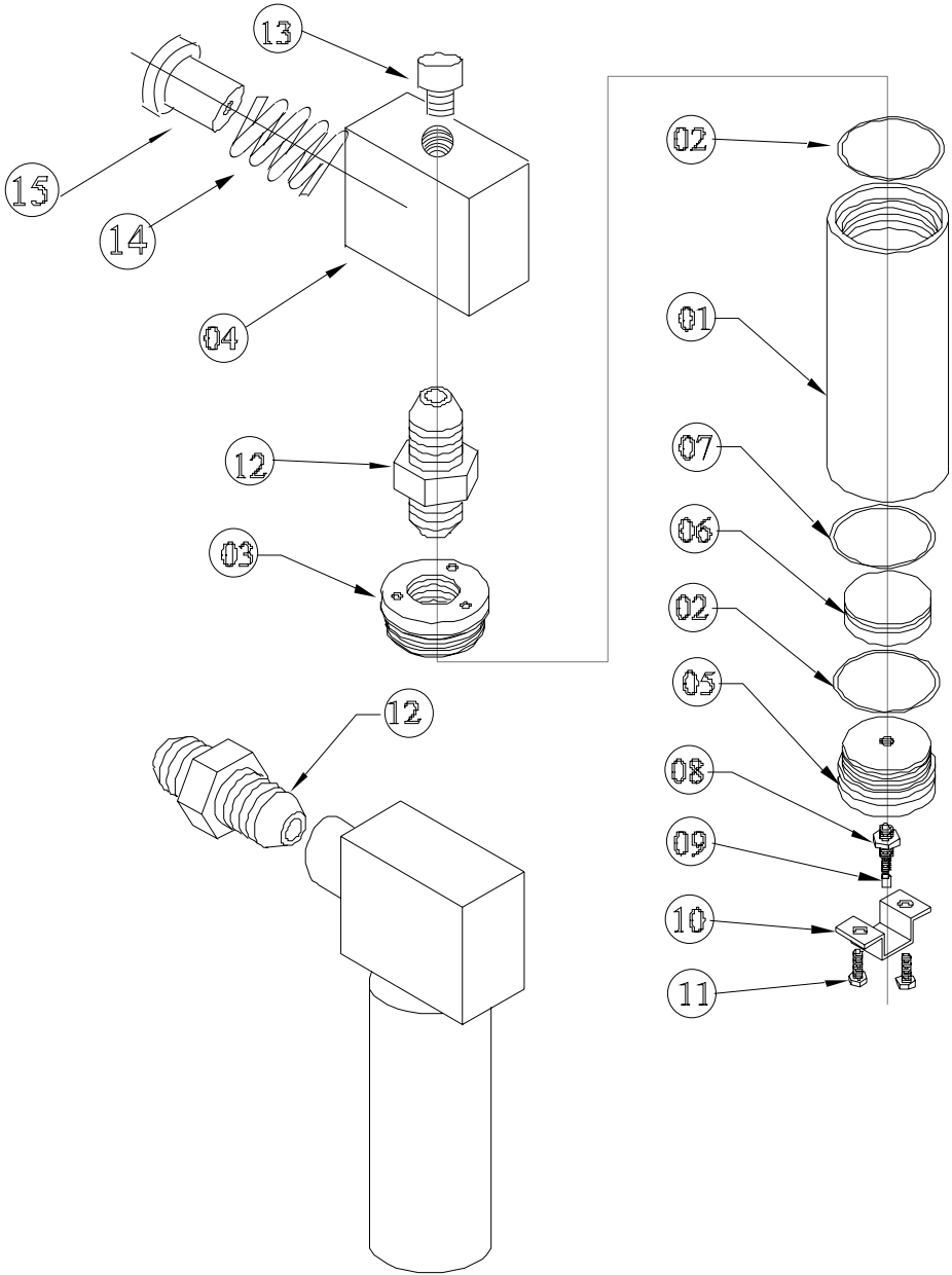
Front Suspension Accumulator
