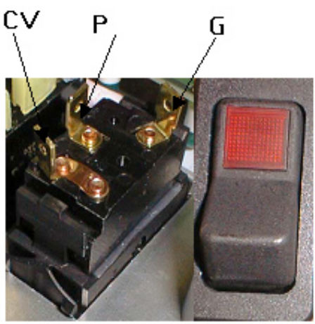
Wire Connections
