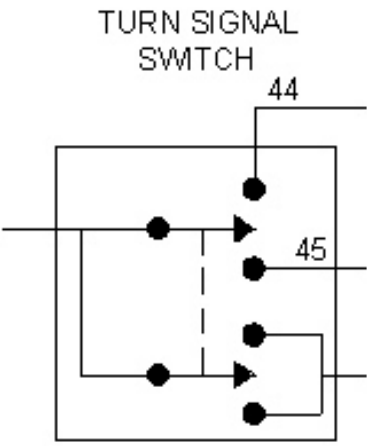
Schematic
