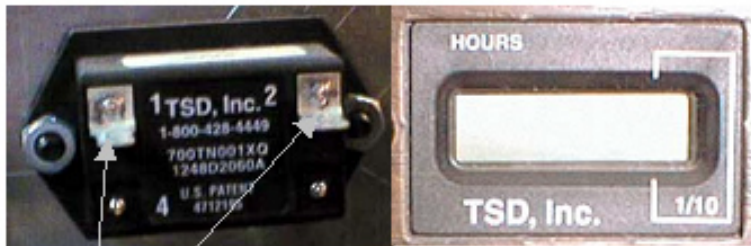
Wire Connections
