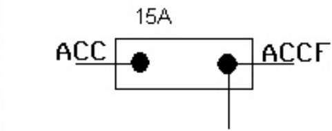
ACCF Schematic
