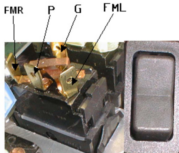
Wire Connections
