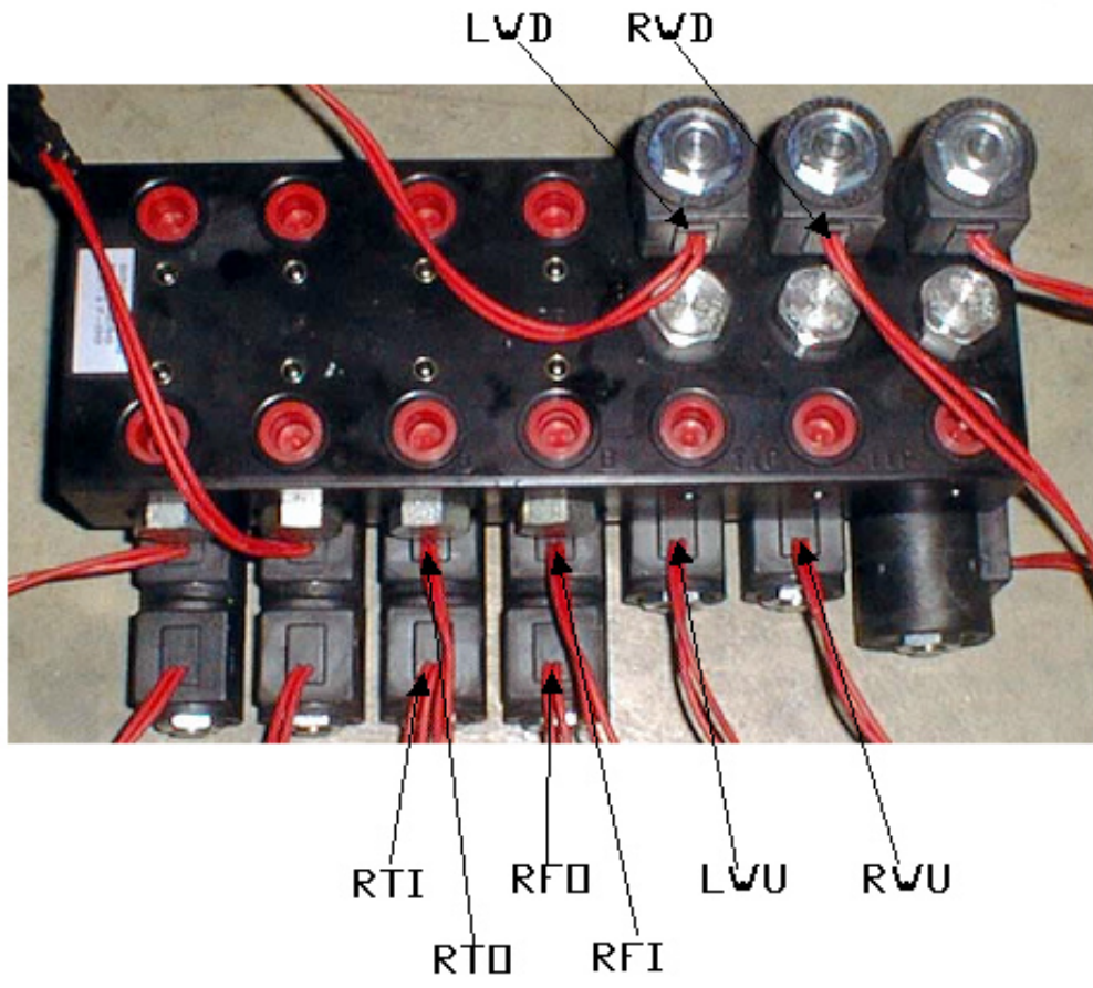
Wire Connections
