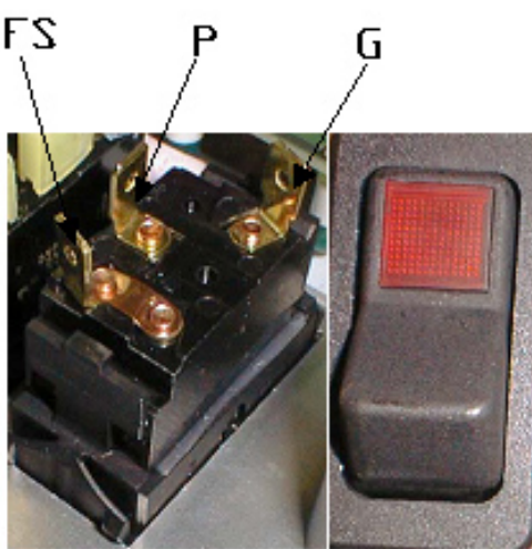
Wire Connections
