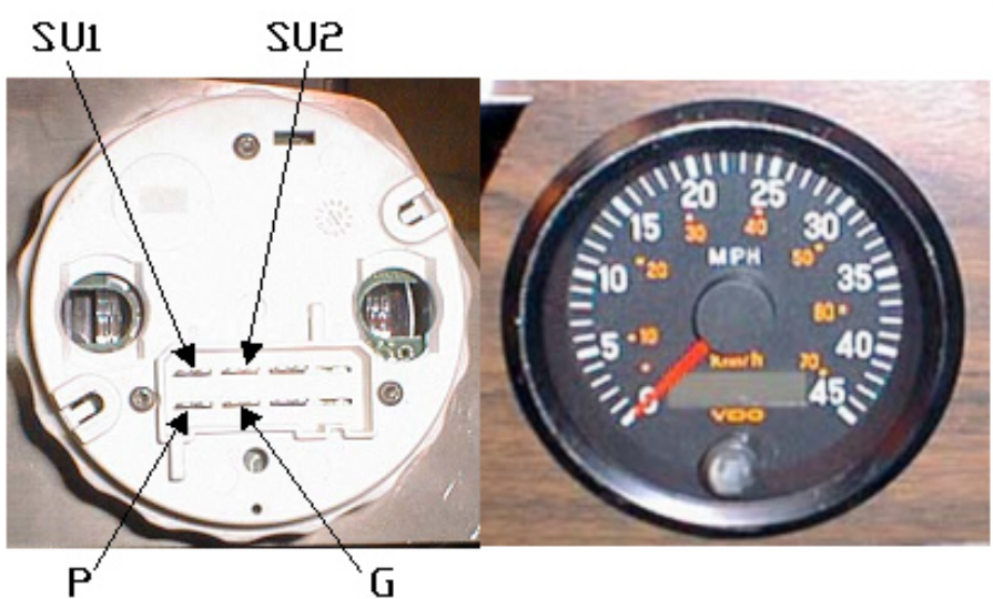
Wire Connections
