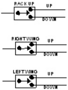
Schematics
