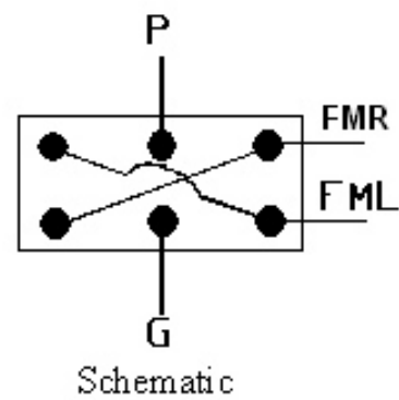
Wire Connections
