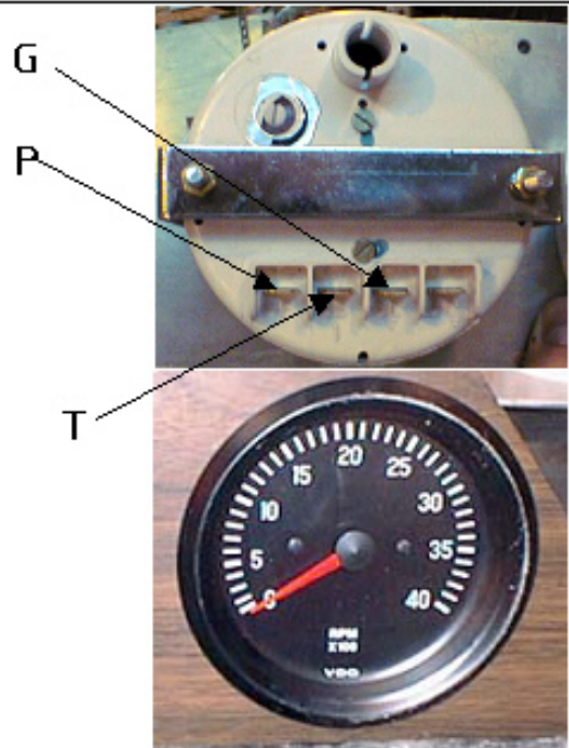
Wire Connections
