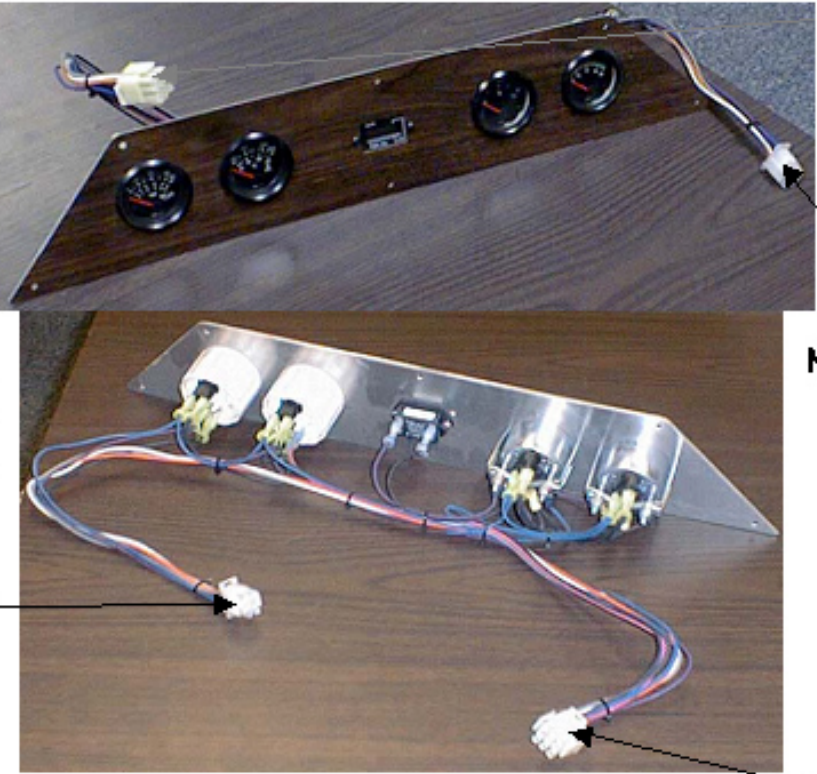
Wire Connections
