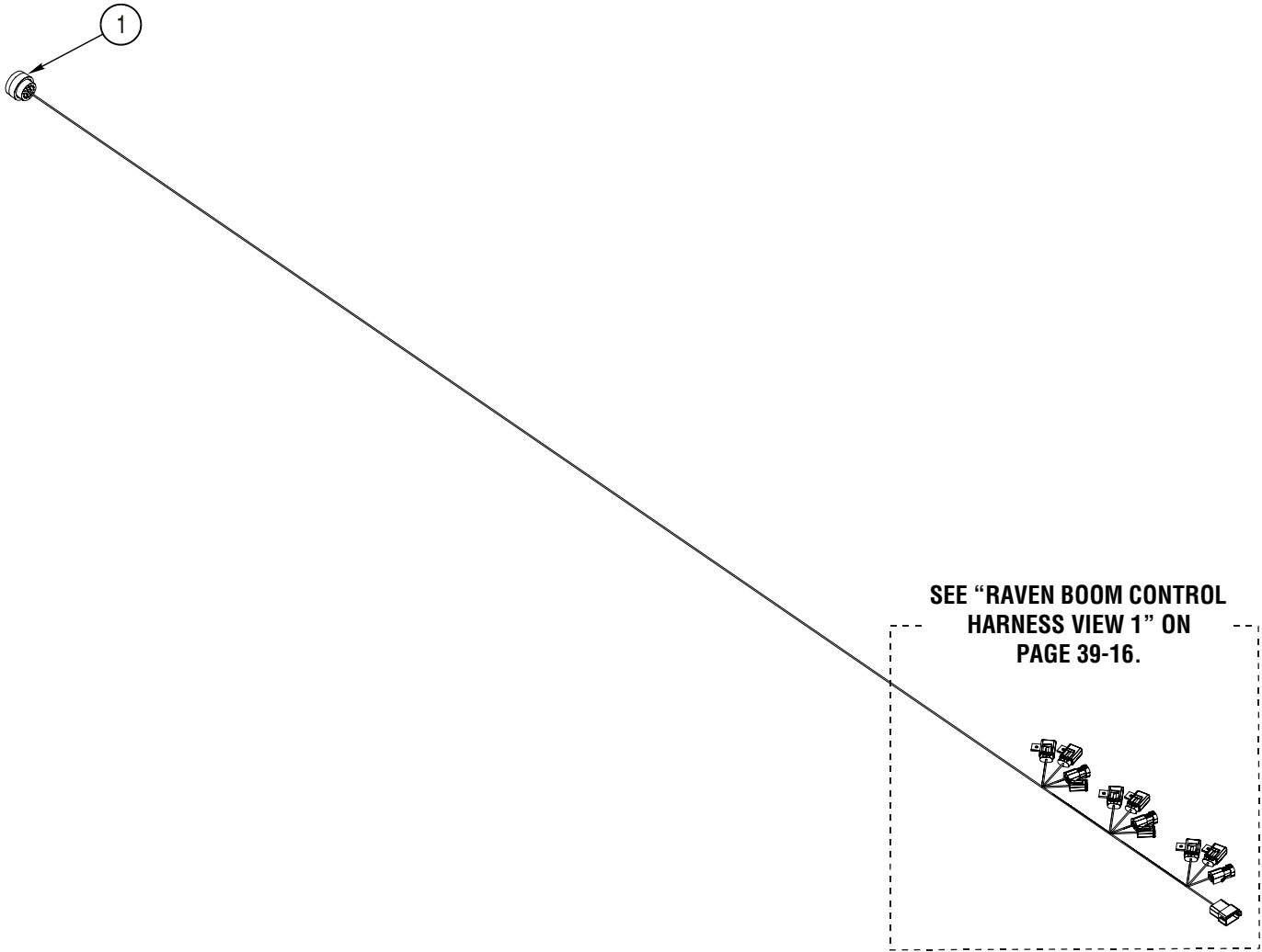
Raven Boom Control Harness Overview
