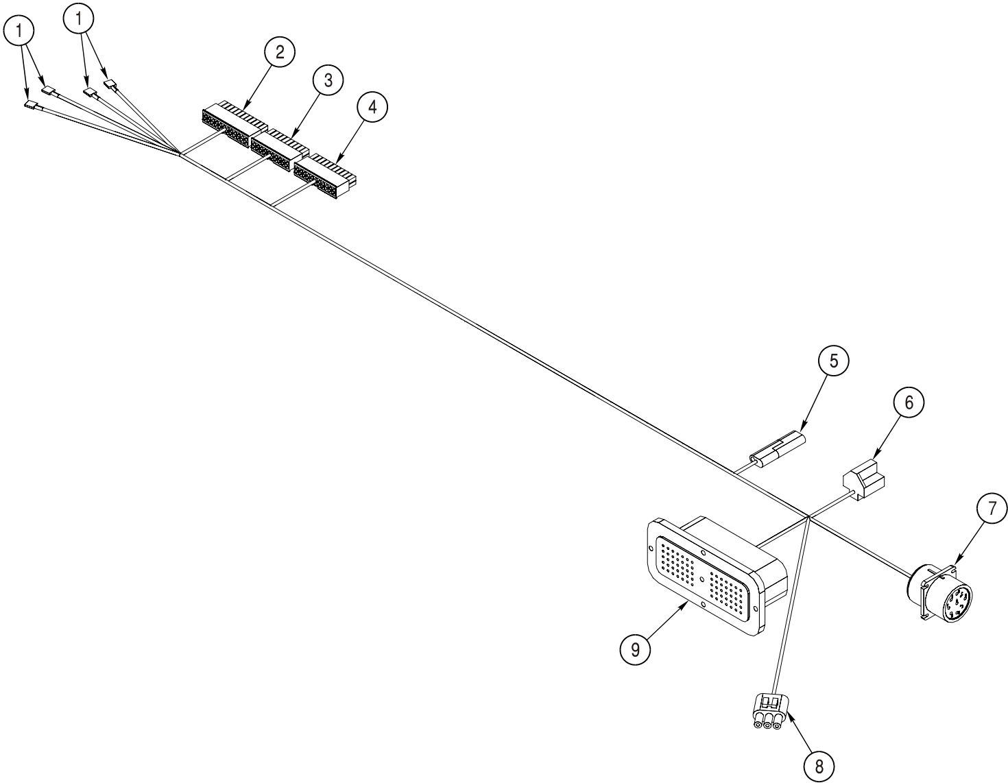
PowerShift 766 Harness
