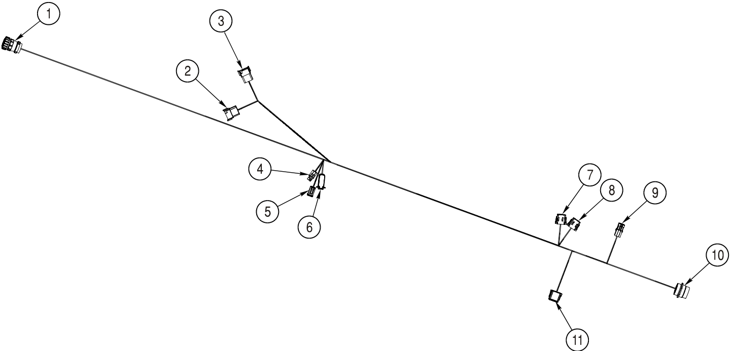
Raven Control Cab Harness
