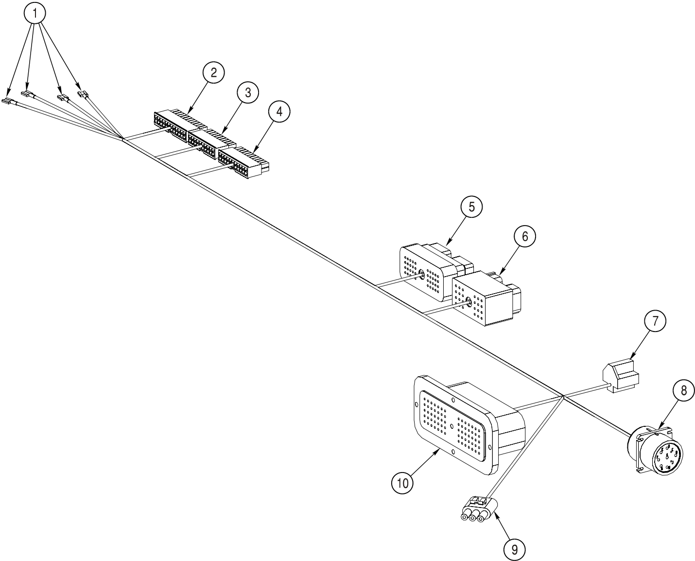
PowerShift 764 Harness
