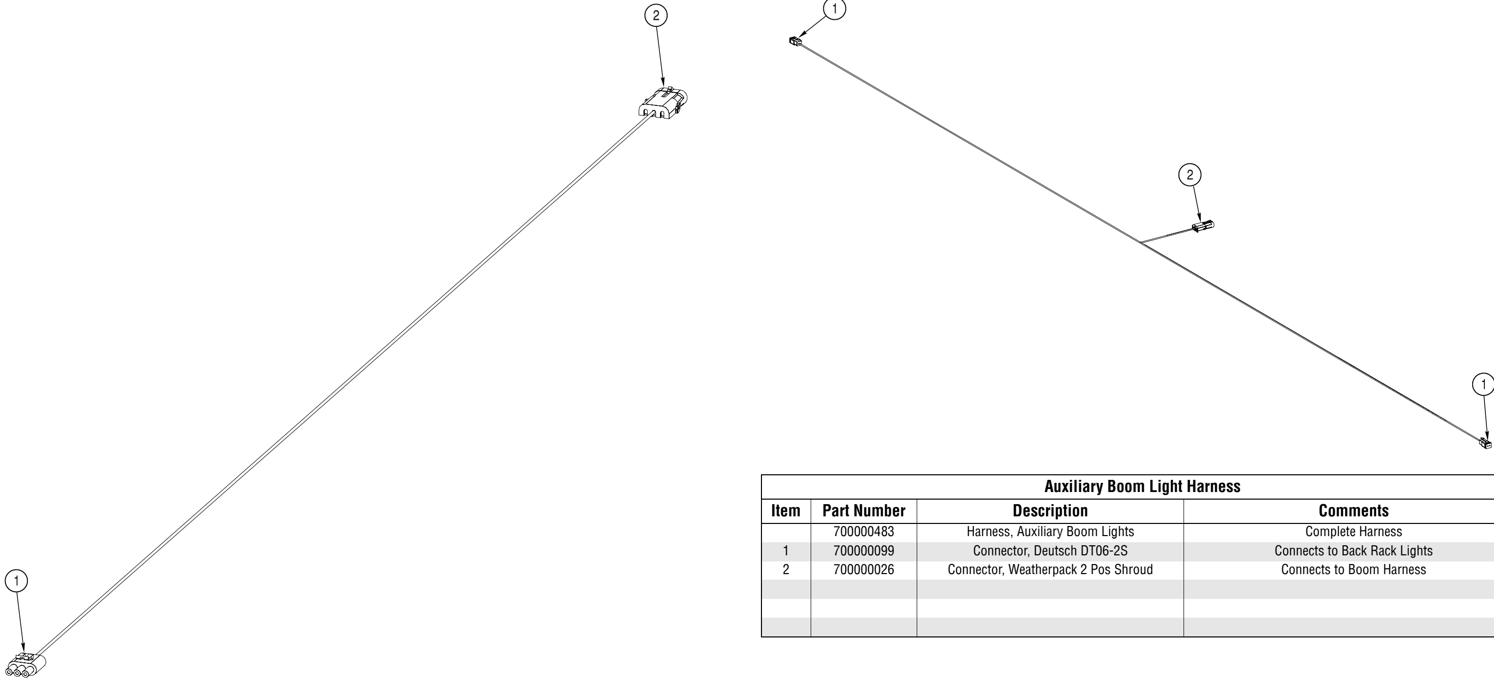
Auxiliary Boom Lights Harness
