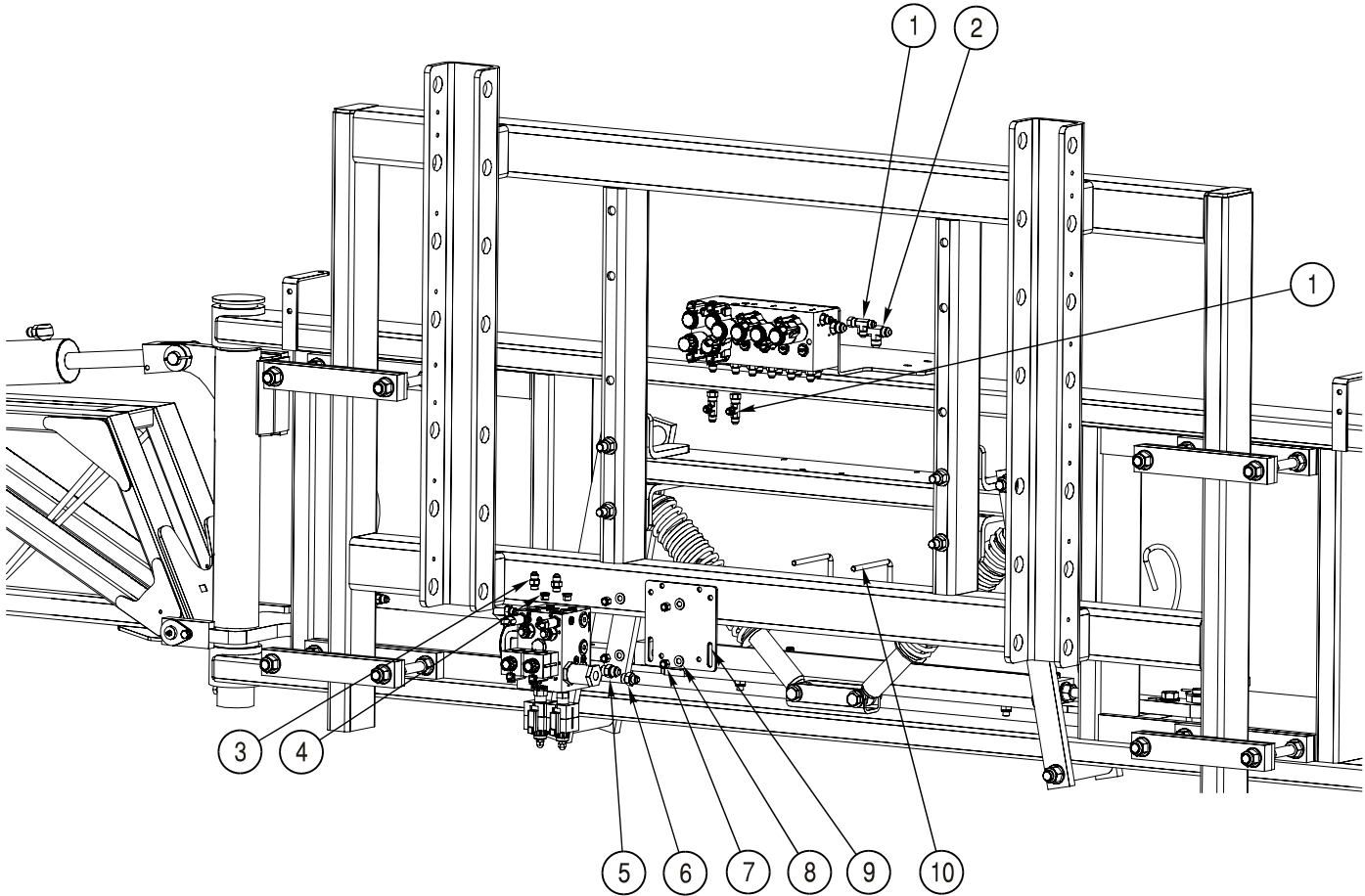
AutoBoom Block & Fitting Layout
