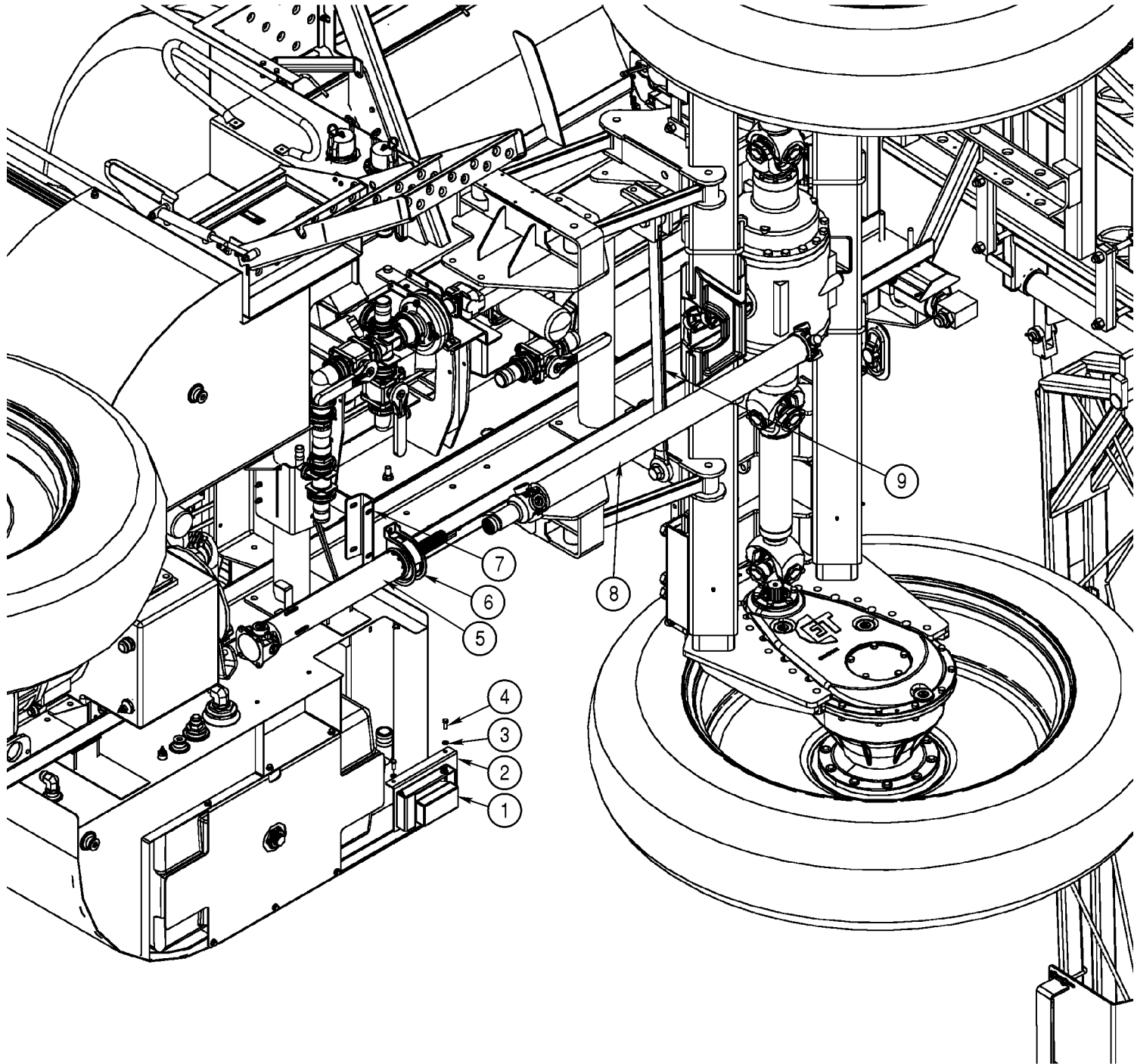
Drive Shaft & Bottom View
