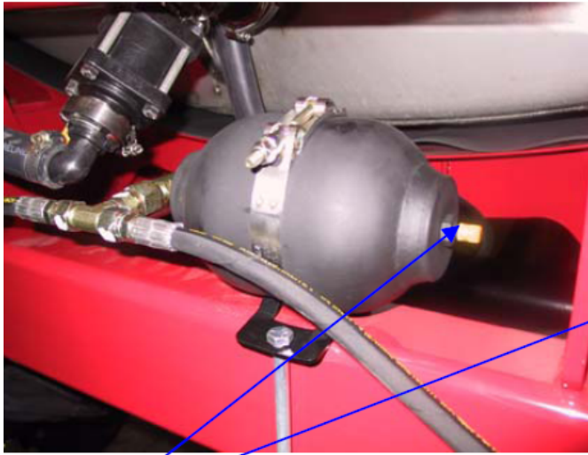
Boom rear center rack accumulator Part# 600901512 version # 1
