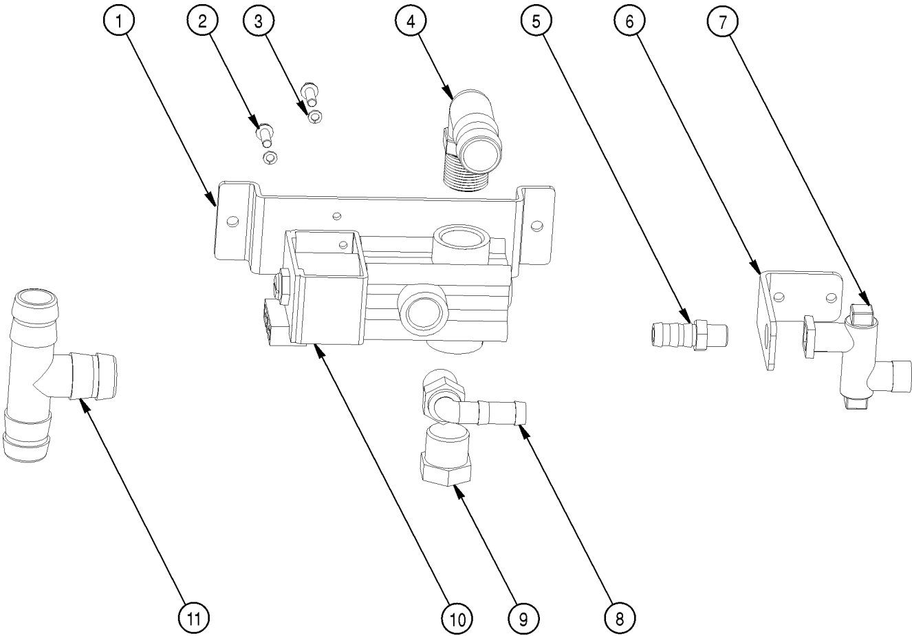
Fencerow Nozzle
